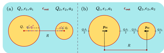
Figure 1. Schematics of the system setup: (a) the reflected Neumann's image charges and (b) the three-point image formula (developed in this work) for two polarizable spheres immersed in a medium. In both panels, tiny colored hollow circles denote image charges, while arrows indicate dipole moments.
