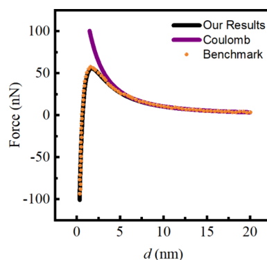
Figure 2. Interaction force between two polarizable spheres in a vacuum as a function of sphere–sphere separation d = R - a_1 - a_2 . Both spheres have a radius of a_1 = a_2 = 1.25 nm, carry central charges of Q_1 = -1e and Q_2 = -7e , and dielectric constants \epsilon_1 = \epsilon_2 = 20 . Black curve: this work; orange dots: benchmark results from ref 44; purple curve: the bare Coulomb interaction between the two spheres.
