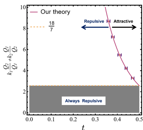
Figure 3. Critical conditions for LCA of two equal-sized spheres predicted by eq 15. For the case \left(k_1 \frac{Q_2}{Q_1} + k_2 \frac{Q_1}{Q_2}\right) > 18/7 , LCA will occur. Purple curve indicates the location of R_c according to eq 15, while each of the error bars (in t ) are obtained from numerical simulations of three different system parameter settings for the same value of \left(k_1 \frac{Q_2}{Q_1} + k_2 \frac{Q_1}{Q_2}\right) (see SI, Table S1 for detailed data). The theory predicts no LCA for \left(k_1 \frac{Q_2}{Q_1} + k_2 \frac{Q_1}{Q_2}\right) \leq 18/7 .
