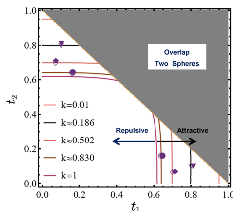
Figure 4. Critical conditions for LCA of two unequal-sized spheres predicted by eq 17, under different values of k ranging from 0.01 to 1. The open and solid symbols represent theoretical and numerical results, respectively, and show an excellent agreement. The upper-right shaded region has no physical meaning due to the non-overlapping constraint t_1 + t_2 \leq 1 .
